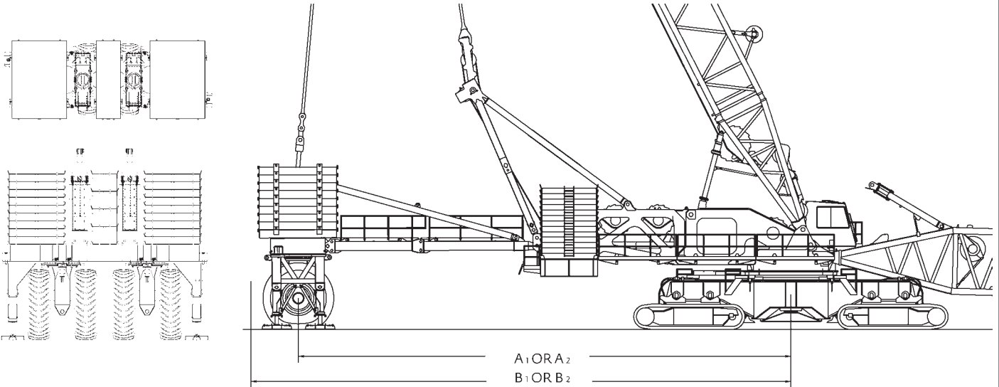
WHEELED COUNTERWEIGHT
